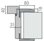
P 208 BİNİLİ KASA STANDART
