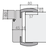
P 108 OTEL KASA OPSİYONEL
