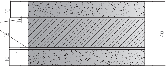
Kurşun Plaka Lead plate
