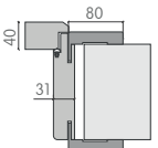
P 005 BİNİLİ KASA STANDART
